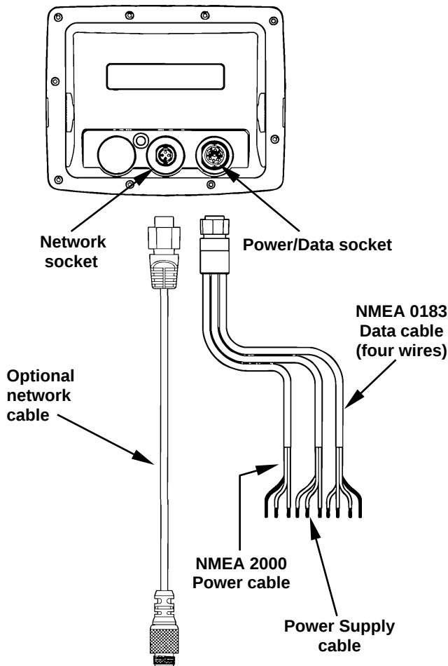
GlobalMap 3600 iGPS Cable Connections.
