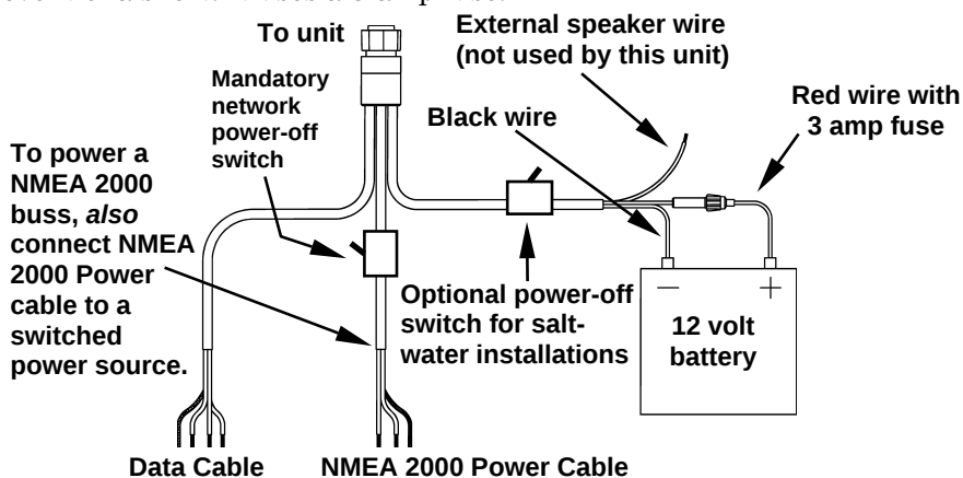
Power connections for GlobalMap 3600C iGPS unit.
