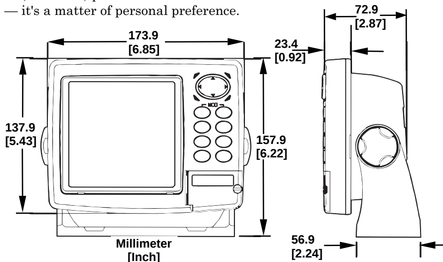
Front view (left) and side view (right) showing dimensions of the GlobalMap 3600C when mounted on gimbal bracket.
