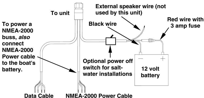
Power connections for the GlobalMap 3500C GPS unit.
