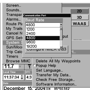
Menus for changing Com Port settings.
