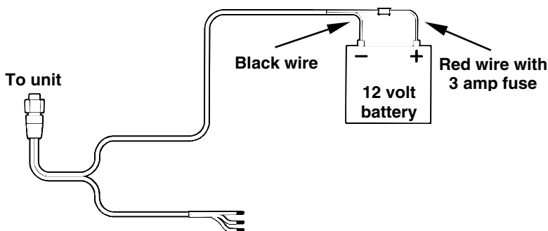
Power connections for the GlobalMap 3200 GPS unit.
